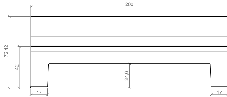
ALZADO / FRONT VIEW
