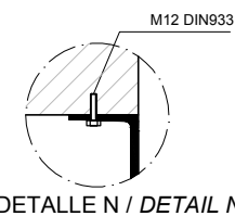
DETALLE N / DETAIL N
