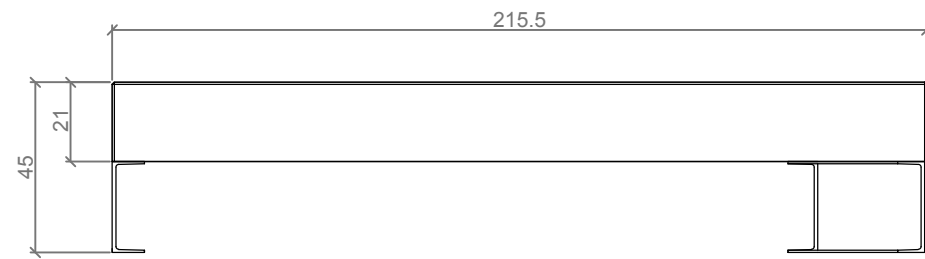
ALZADO / FRONT VIEW
