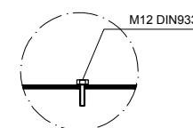
DETALLE M / DETAIL M
