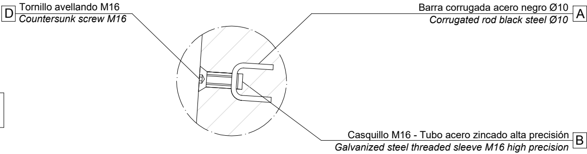
DETALLE M / DETAIL M
