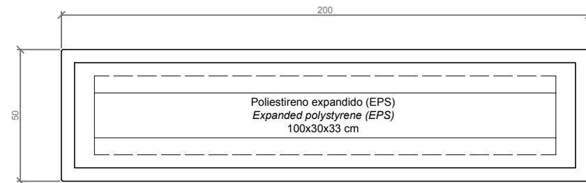
VISTA INFERIOR / BOTTOM VIEW
