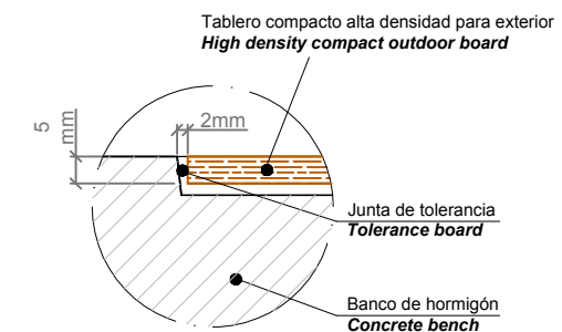
DETALLE 1 DETAIL 1
