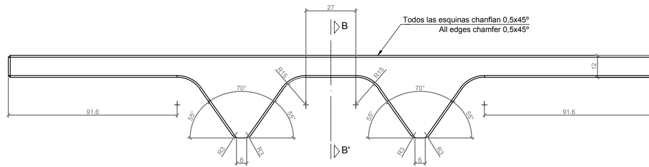
ALZADO / FRONT VIEW
