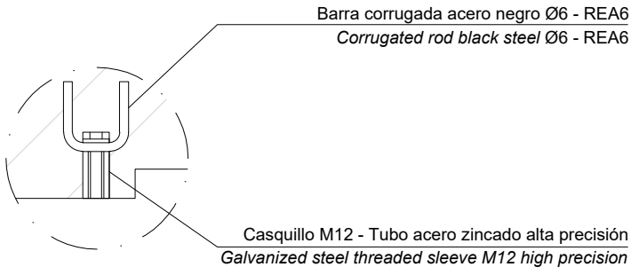
DETALLE B / DETAIL B
