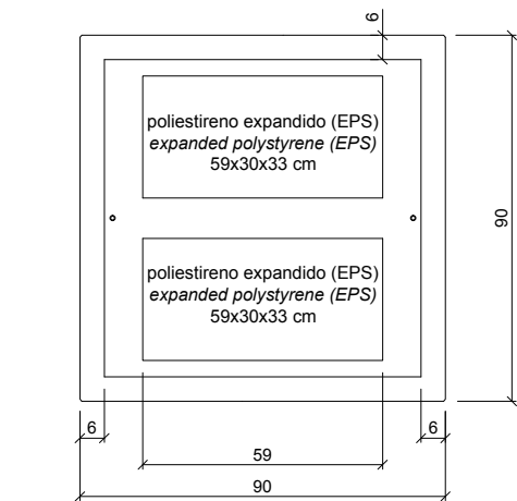
VISTA INFERIOR / BOTTOM VIEW
