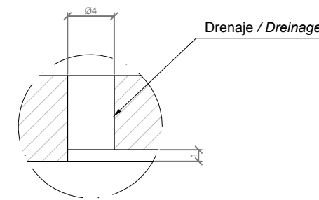
DETALLE M / DETAIL M
