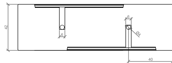
VISTA INFERIOR / BOTTOM VIEW
