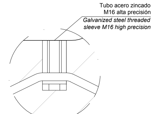
DETALLE C / DETAIL C
