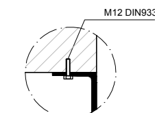
DETALLE N / DETAIL N
