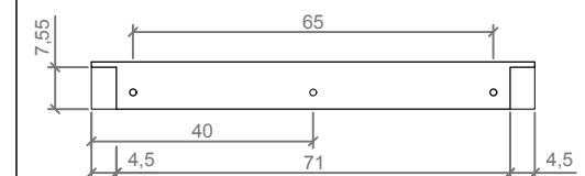
DETALLE N / DETAIL N
