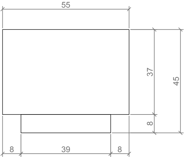
ALZADO / FRONT VIEW
