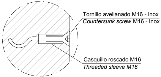
DETALLE M - DETAIL M
