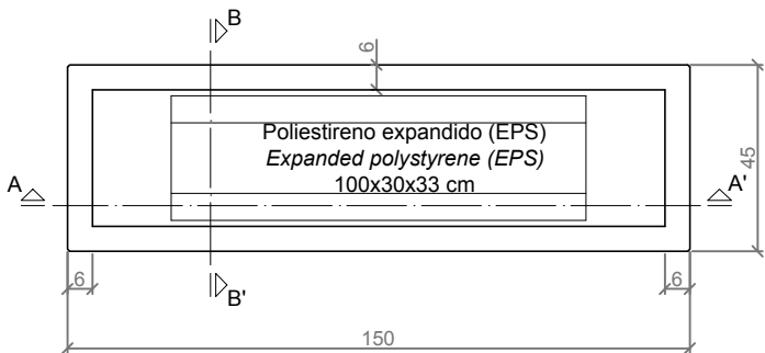
VISTA INFERIOR / BOTTOM VIEW
