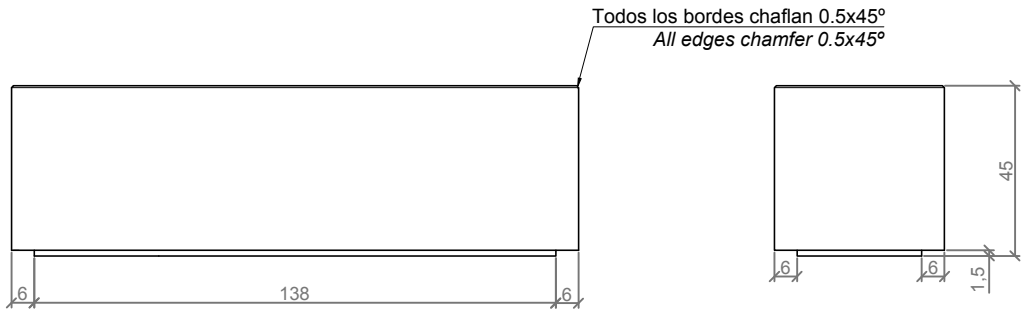
ALZADO / FRONT VIEW
