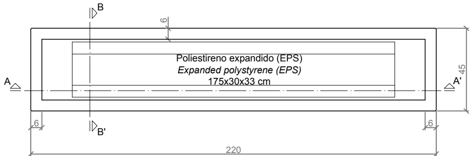
VISTA INFERIOR / BOTTOM VIEW
