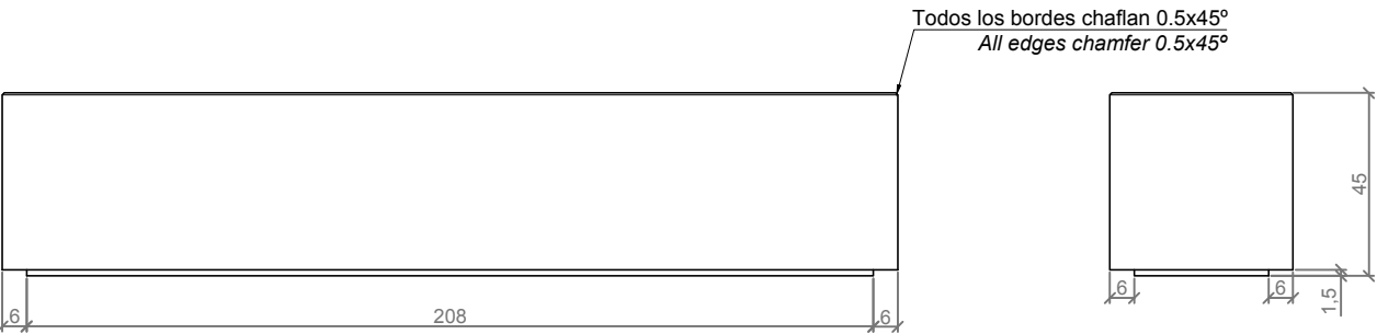
ALZADO / FRONT VIEW
