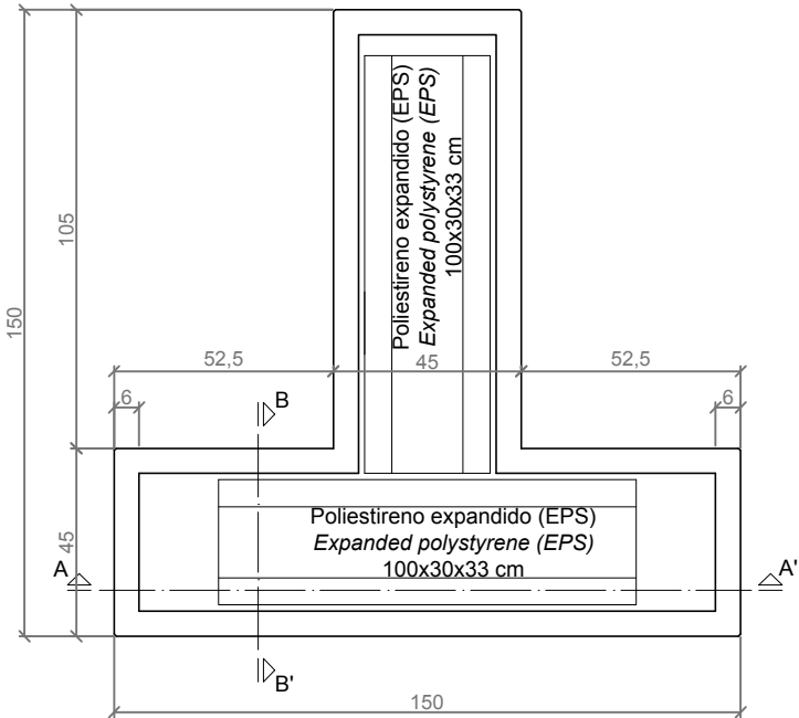
VISTA INFERIOR / BOTTOM VIEW
