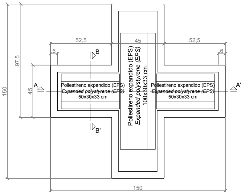
VISTA INFERIOR / BOTTOM VIEW
