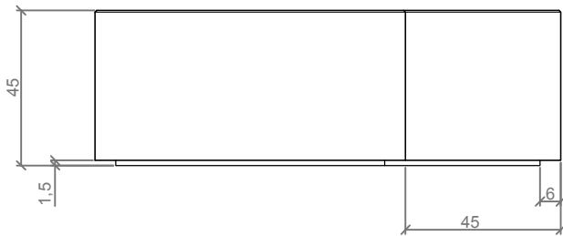
ALZADO / FRONT VIEW
