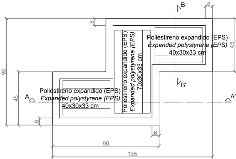
VISTA INFERIOR / BOTTOM VIEW
