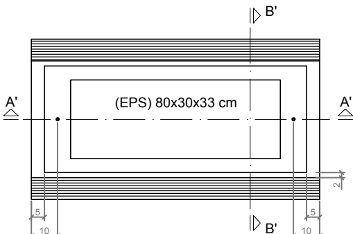
VISTA INFERIOR / BOTTOM VIEW
