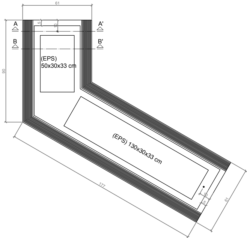
VISTA INFERIOR / BOTTOM VIEW
