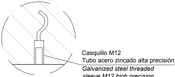
DETALLE B / DETAIL B
