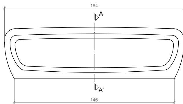
ALZADO / FRONT VIEW
