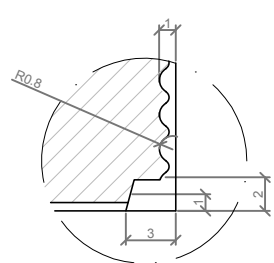
DETALLE N / DETAIL N
