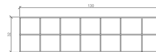
DETALLE F / DETAIL F
