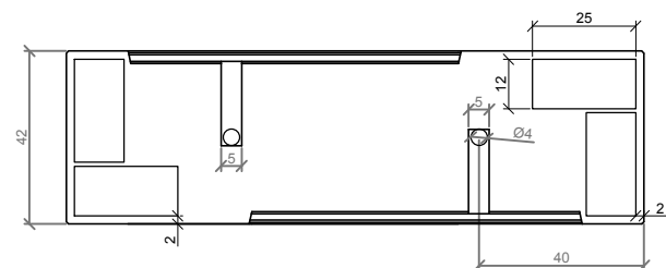
VISTA INFERIOR / BOTTOM VIEW
