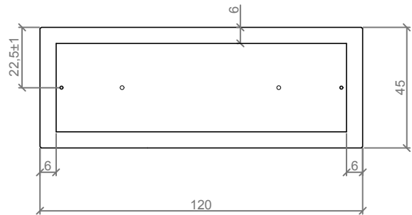
VISTA INFERIOR / BOTTOM VIEW
