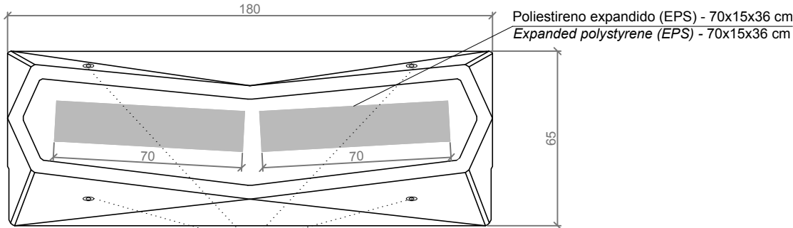
VISTA INFERIOR / BOTTOM VIEW
