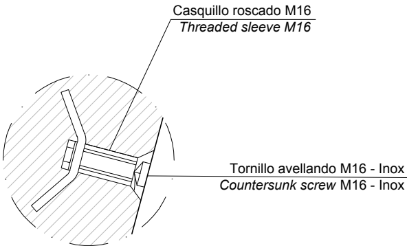
DETALLE N / DETAIL N
