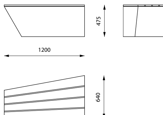
CRO-A2-W 340 kg
